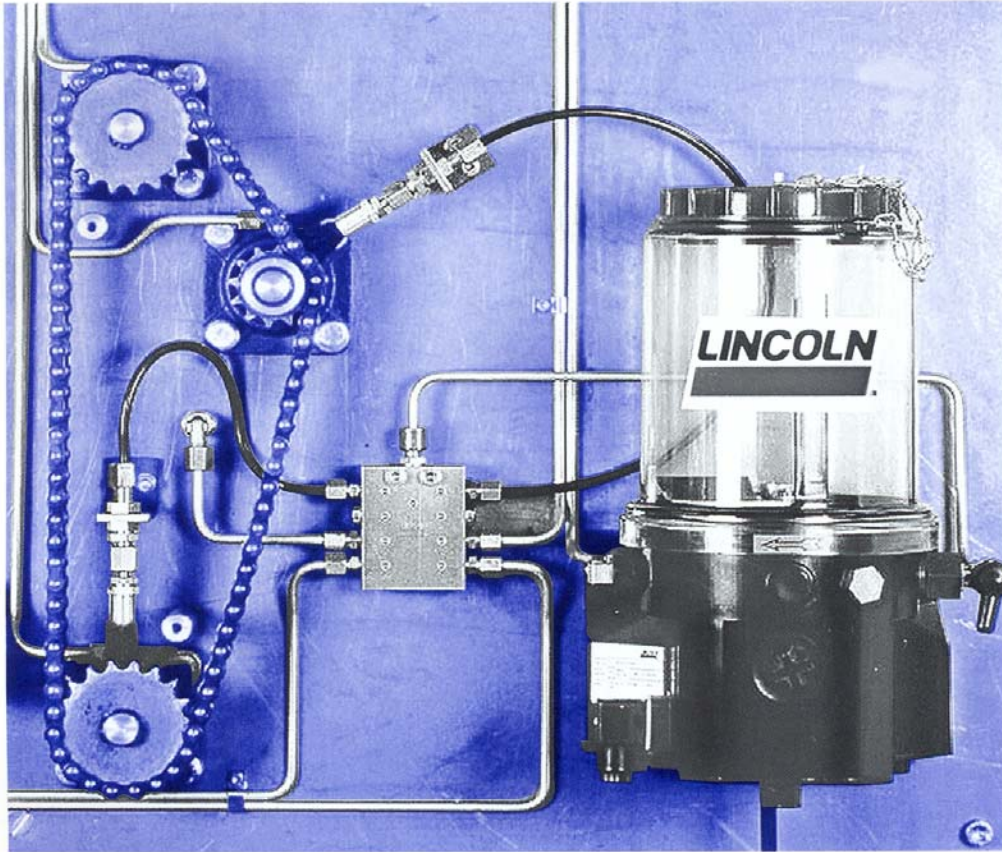
Chain Lubrication
